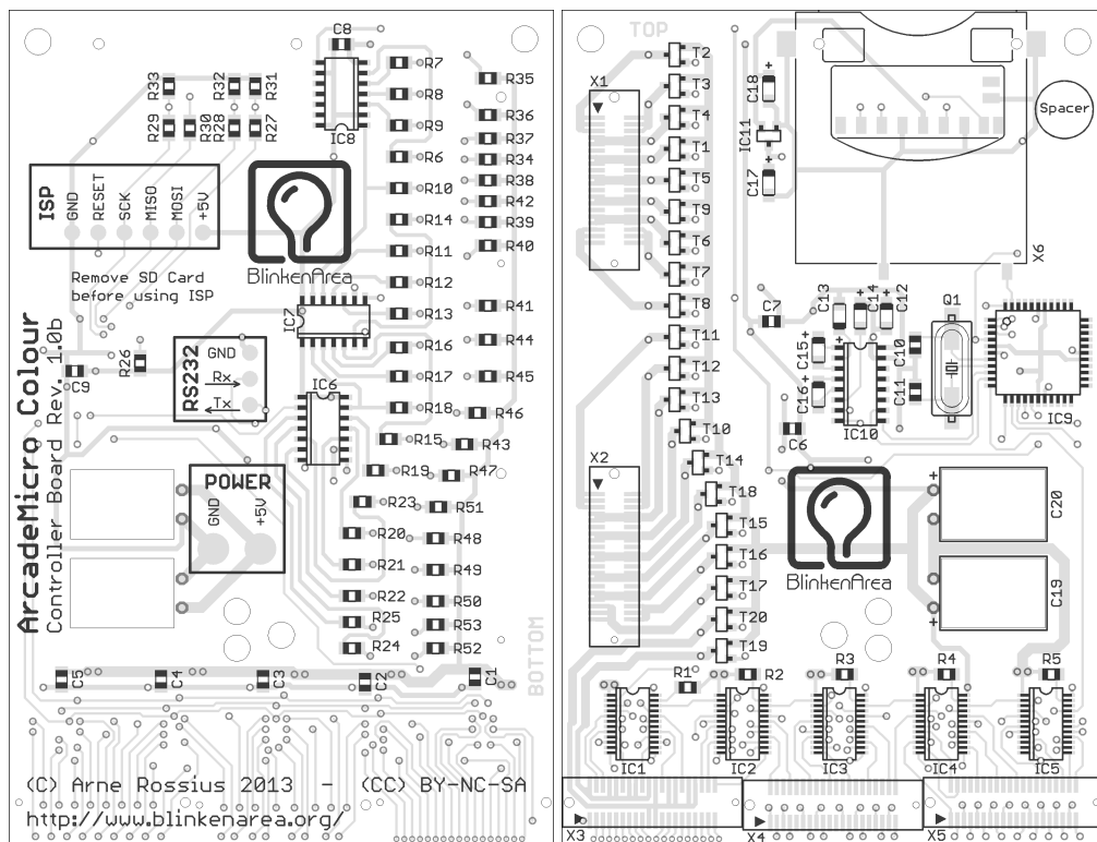
Controller Board, Top Side
